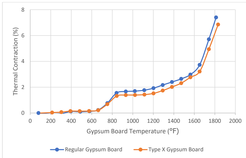
Figure C3-9. Thermal Contraction of Gypsum Board
