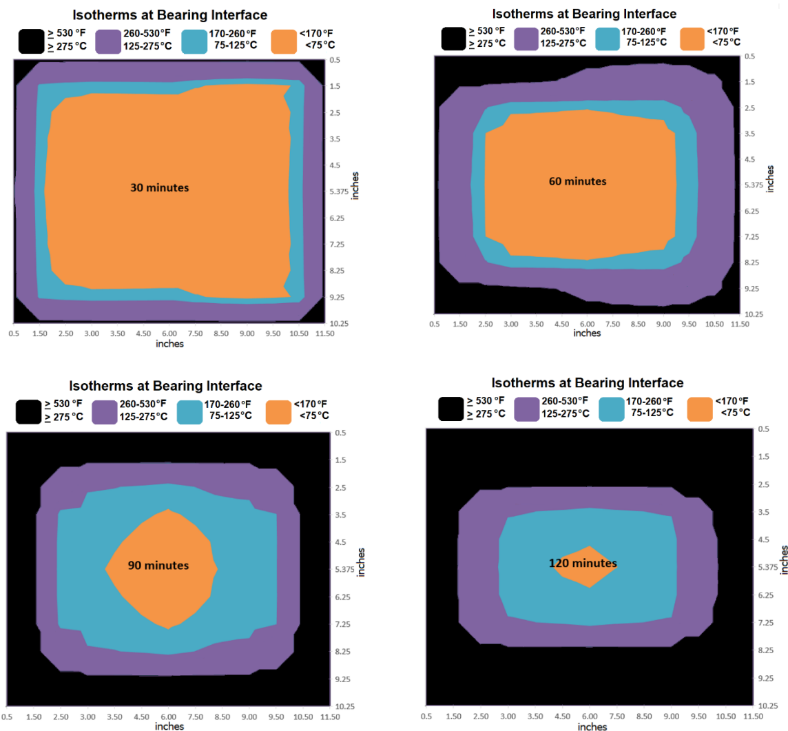
Figure C3-6 Isotherms at Bearing Interface
