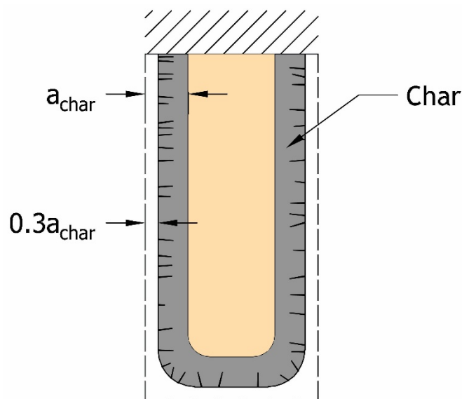
Figure 1-3. Char contraction
