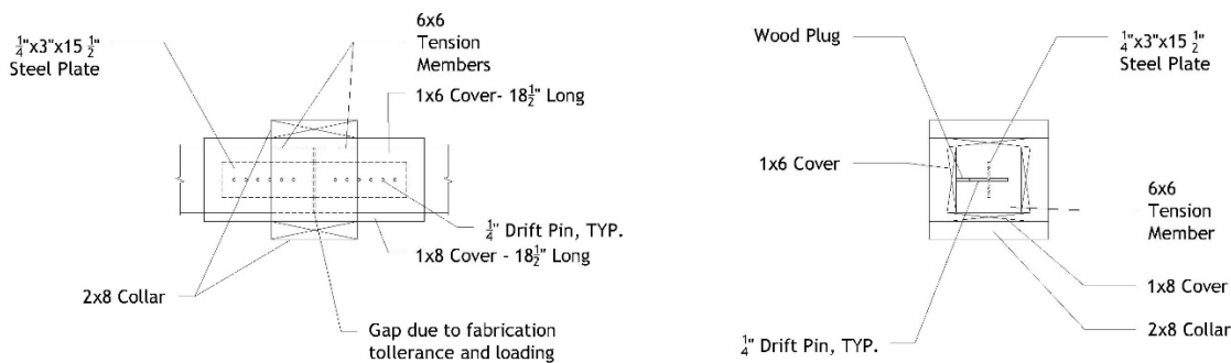
Figure 10-5. Final wood protection design
