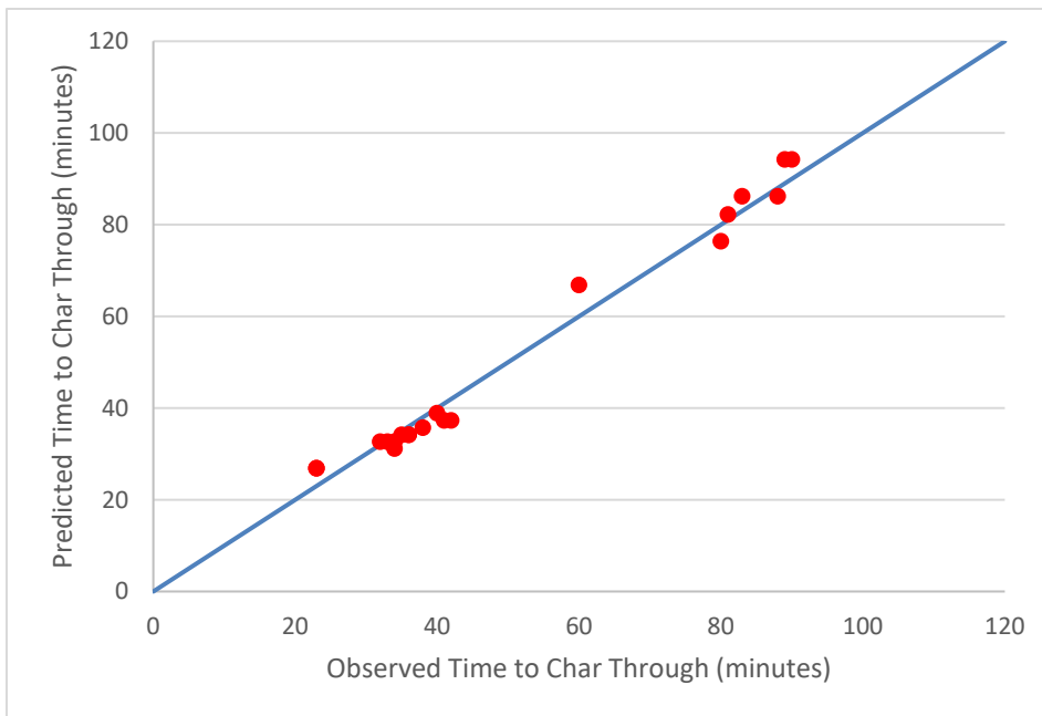
Figure 3-3 Comparison of Predicted to Observed Time to Char Through (Unprotected Rimboard)
