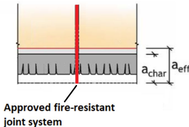
Figure 1-10. Example showing approved fire-resistant joint system on the exposed side.
