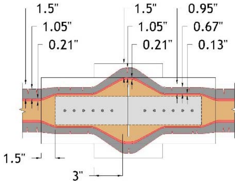
Figure 10-4. Char pattern and calculated dimensions including the effects of char penetration
