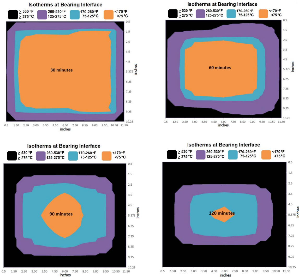
Figure 1-3. Isotherms at bearing interface
