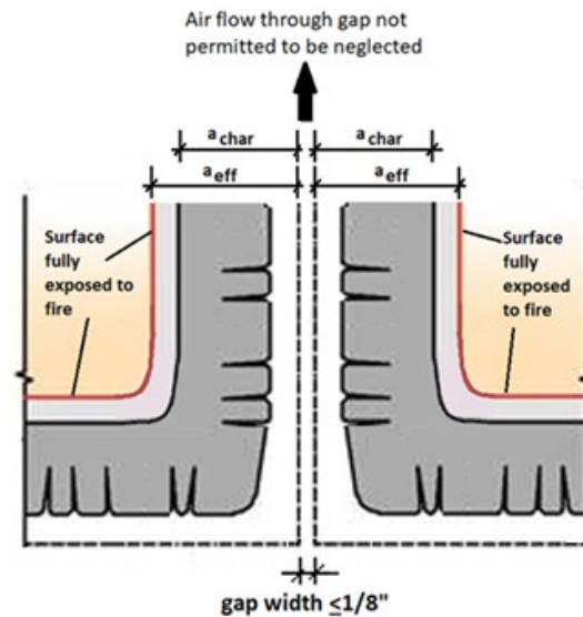
Figure 1-9. Example showing char penetration where gap is less than or equal to 1/8-inch on the exposed side and where air flow is not permitted to be neglected.
