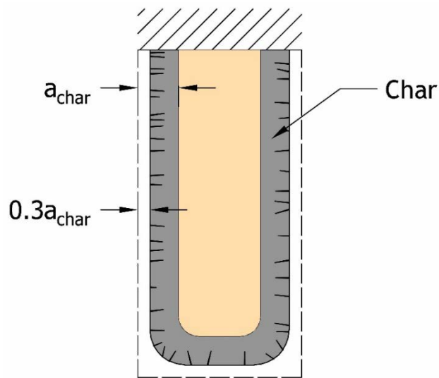
Figure 1-4. Char contraction
