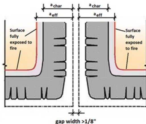
Figure 1-8. Example showing char penetration where gap is greater than 1/8-inch on the exposed side.
