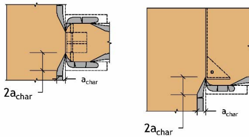
Figure 9-3. Char pattern due to char penetration
