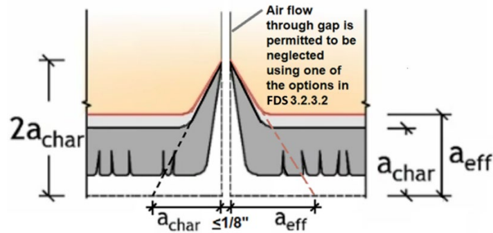
Figure 1-7. Example showing char penetration where gap is less than or equal to 1/8-inch on the exposed side and where air flow through gap is permitted to be neglected.
