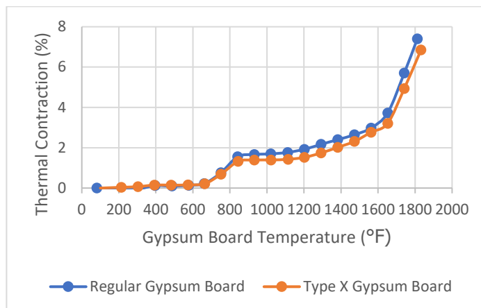
Figure C3-9. Thermal Contraction of Gypsum Board
