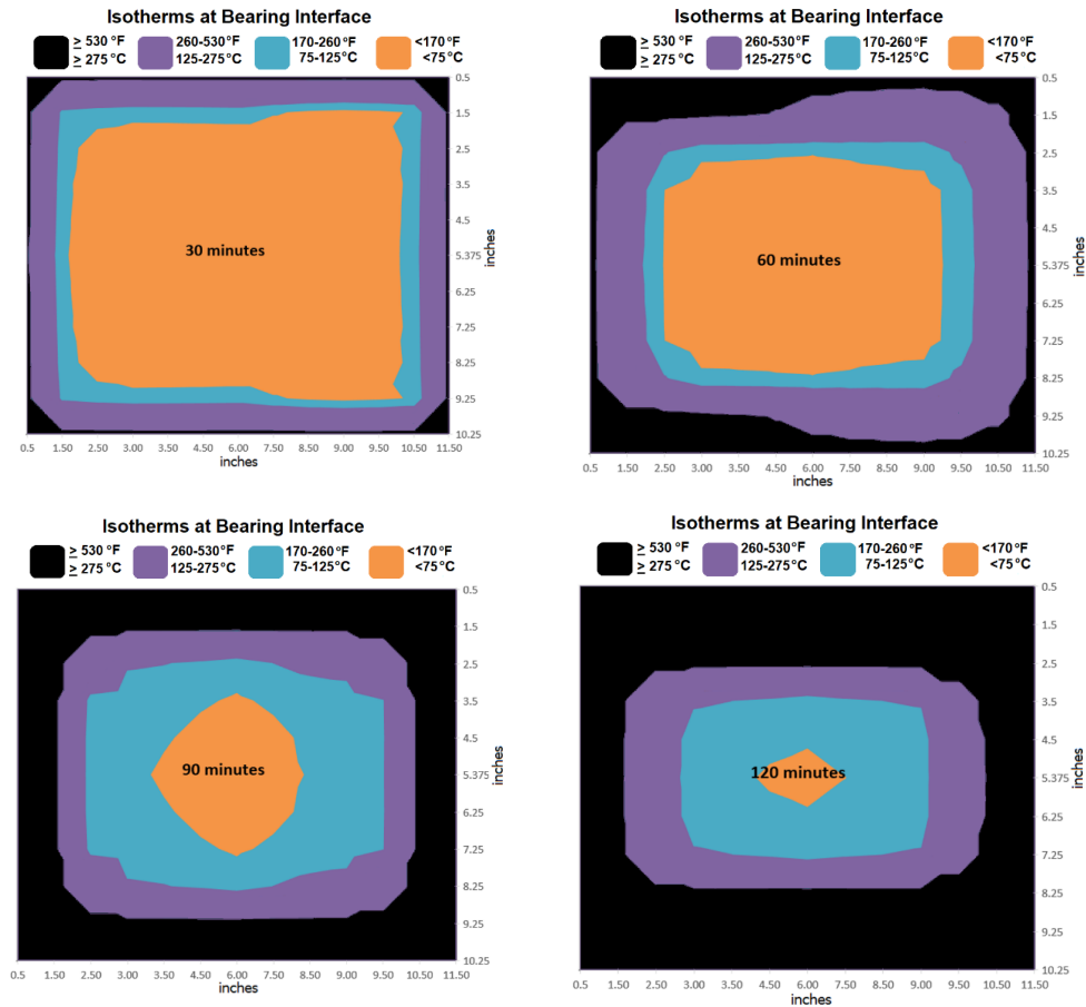
Figure C3-6 Isotherms at Bearing Interface
