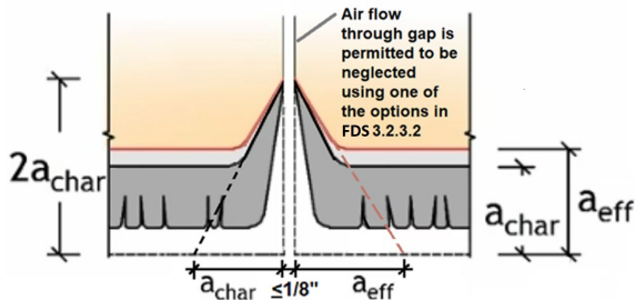
Figure C3-7 Example showing char penetration for decking where gaps are obstructed
