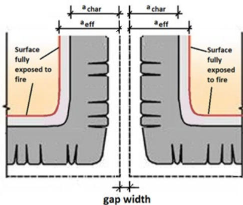
Figure C3-8 Example showing char penetration for decking where gaps are unobstructed
