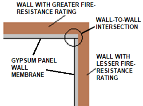
FIGURE C1-3 Gypsum panel wall membrane installation at wall-to-wall intersection
