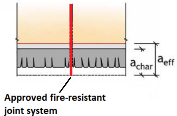
Figure C3-2 Example showing approved fire-resistant joint system on the exposed side
