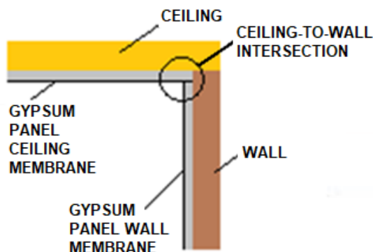
FIGURE C1-2 Gypsum panel ceiling and wall membrane installation at ceiling-to-wall intersection
