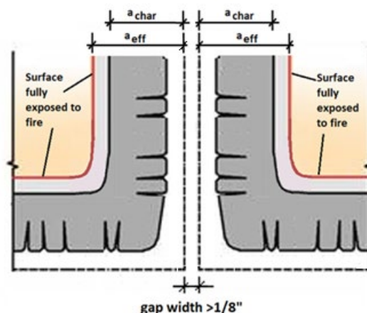
Figure C3-5 Example showing char penetration where gap is greater than 1/8-inch on the exposed side
