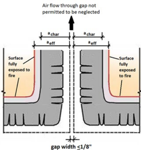
Figure C3-4 Example showing char penetration where gap is less than or equal to 1/8-inch on the exposed side and where air flow is not permitted to be neglected
