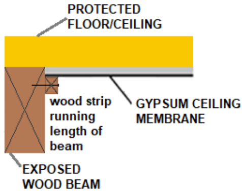
FIGURE C1-1 Example of a gypsum ceiling membrane abutting an exposed wood beam.
