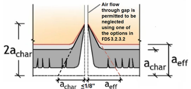
Figure C3-3 Example showing char penetration where gap is less than or equal to 1/8-inch on the exposed side and where air flow through gap is permitted to be neglected
