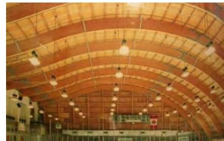
Figure 20: Heavy Timber Construction
