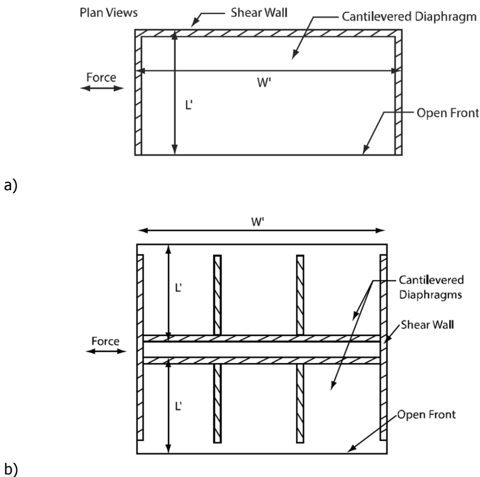
Figure 3. Excerpt from 2015 SDPWS new Figure 4A showing examples of open front structures. In this case, an example of a) a simple open front structure with walls on three sides only and b) a simple corridor wall structure.
