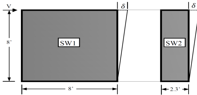
Figure 5. Distribution of shear to shear walls in a line to produce equal deflection in each shear wall is the underlying basis of the familiar 2b_s/h factor
