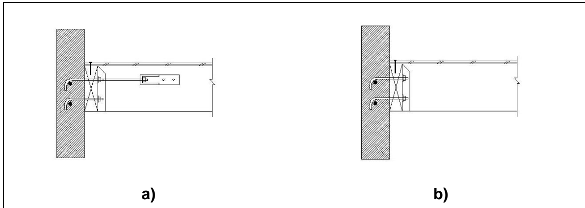
Figure 2. a) Appropriate wall anchor detail where anchor forces are transferred directly into diaphragm framing, and b) wall anchor detail where anchor forces induce cross grain bending in the wood ledger (not permitted).
